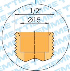
Art. 1717 Per tubo Pe-x For Pe-x pipe
